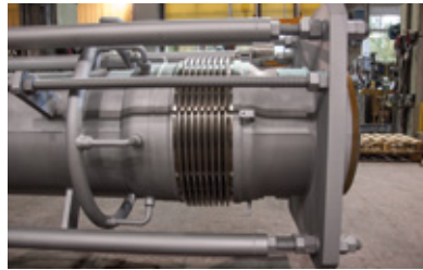
The ring line is positioned behind the inner bellows protective tube. Easily recognisable: the bellows segment with larger diameter
